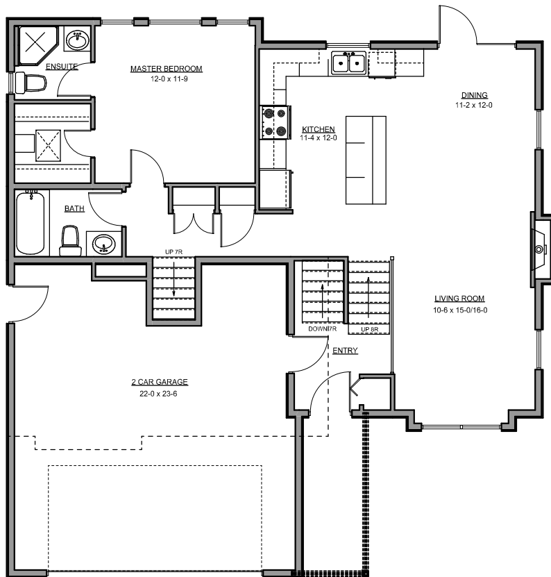
MAIN FLOOR PLAN 921 SQ FT
