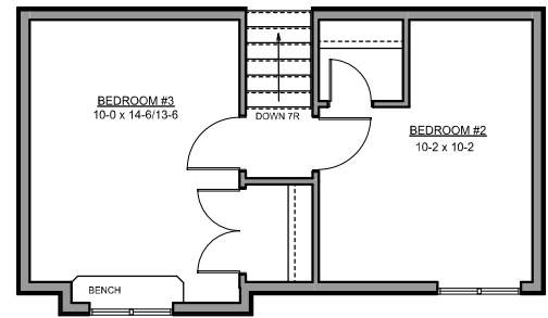
UPPER FLOOR PLAN 347 SQ FT
