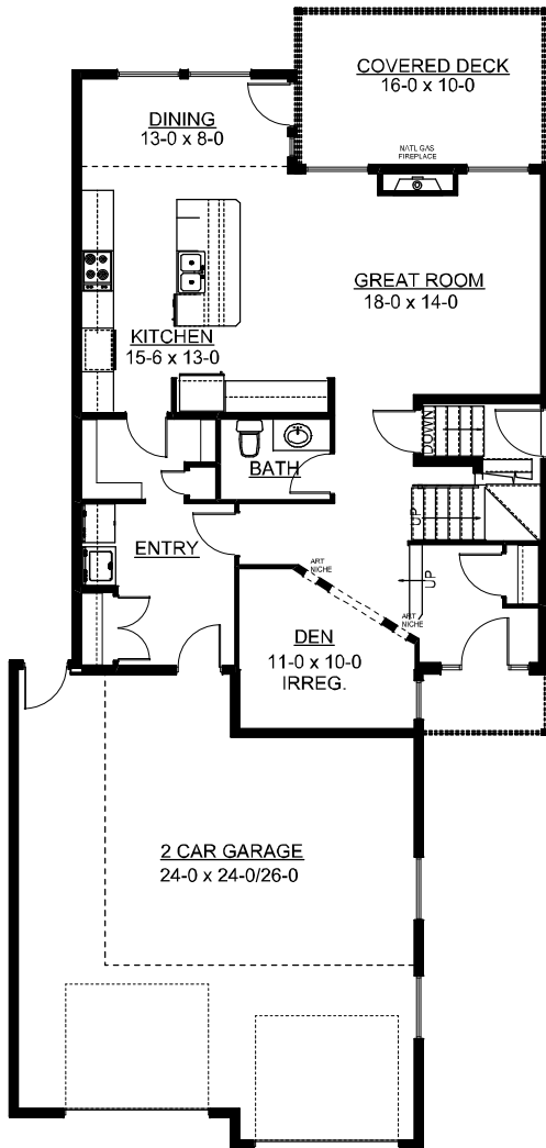
MAIN FLOOR PLAN 1092 SQ FT
