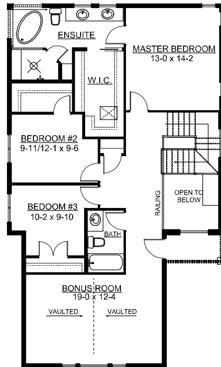
UPPER FLOOR PLAN 1263 SQ FT
